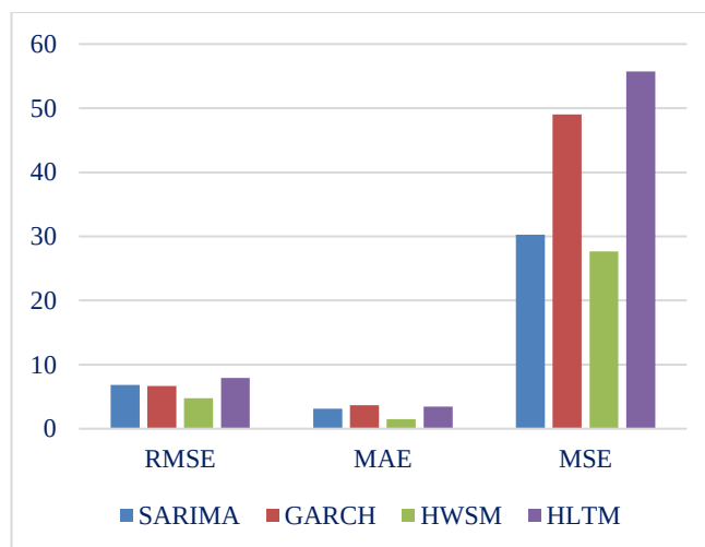
Fig. 4: Forecasting models of MAE, MSE and RMSE values of Dataset - 1
